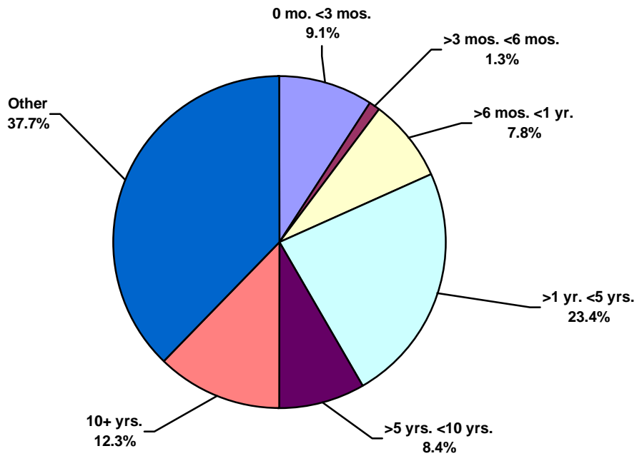
Africa Water Total Recordable Incidents by Time in Service (Chart 16) Based on 154 Incidents
